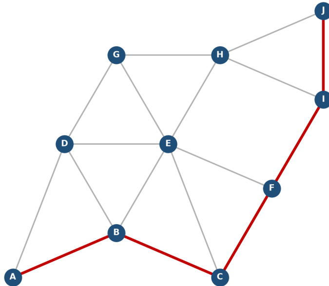
Road-network graph; red = A* recommended route A→B→C→F→I→J
